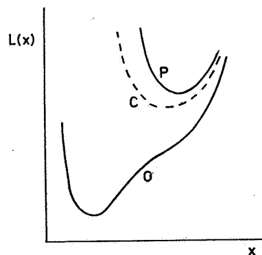
Fig. 1. Extreme estimates of the loss function
